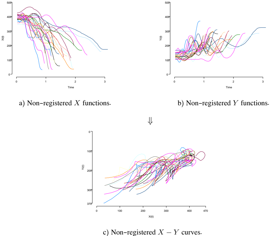
Figure 4. Non-registered data.
